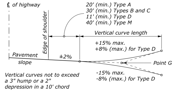
PROFILE OF TYPE A, B, C, D, M APPROACHES
