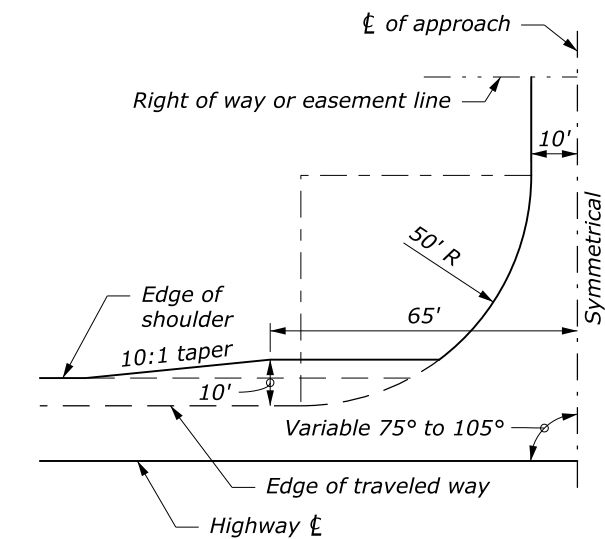
PLAN OF TYPE C APPROACH
