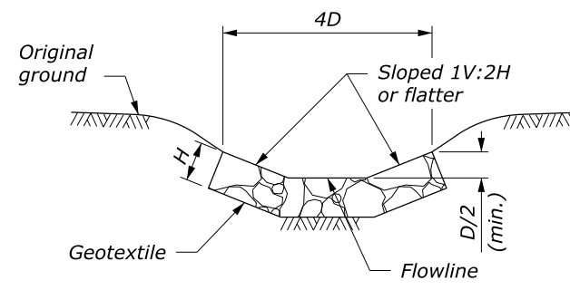
SECTION E-E
