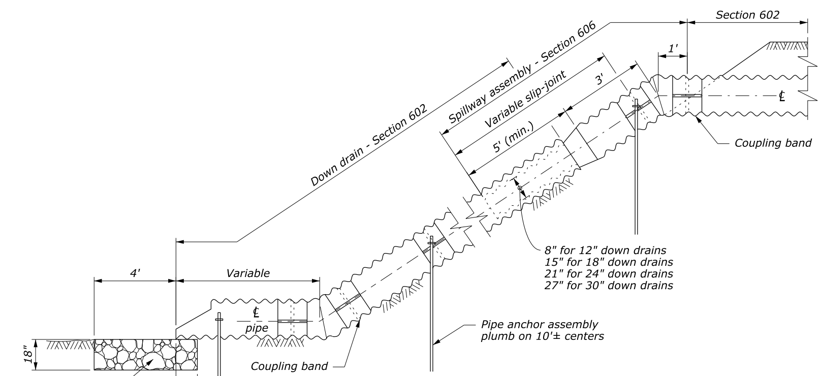
SPILLWAY ASSEMBLY WITH BURIED DOWN DRAIN
