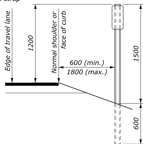
TYPICAL INSTALLATION
