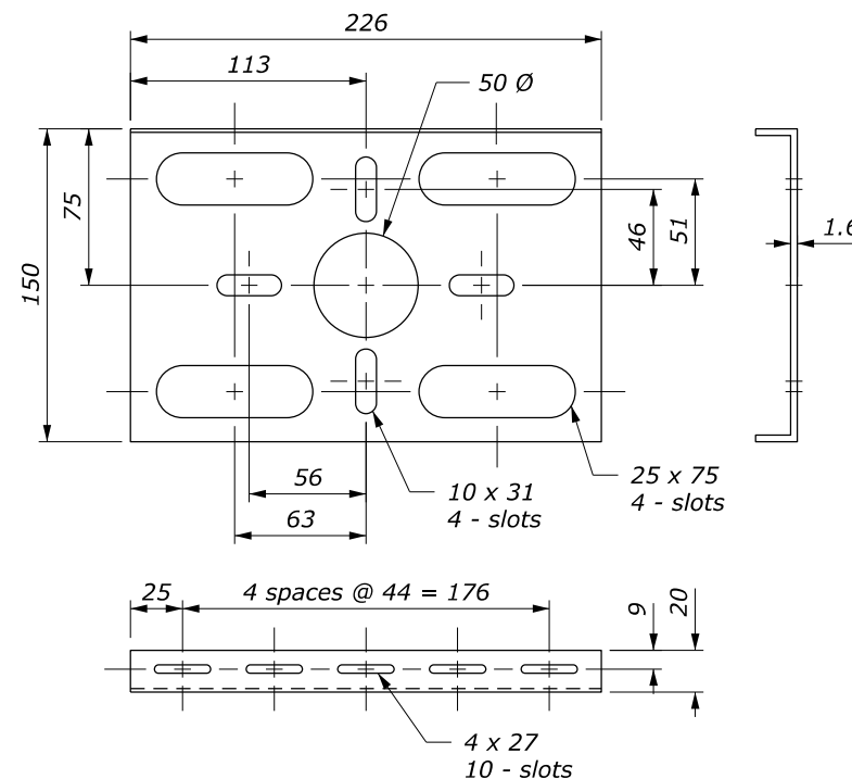
PLATFORM
