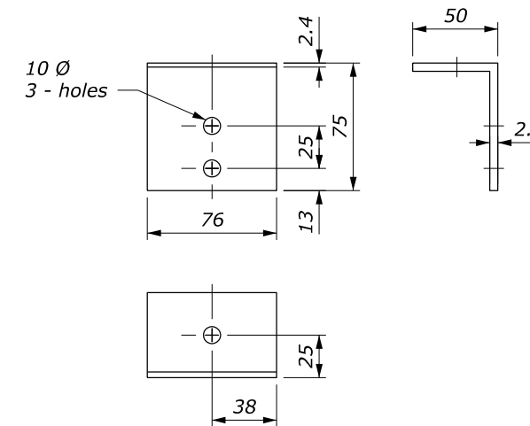
BRACKET
