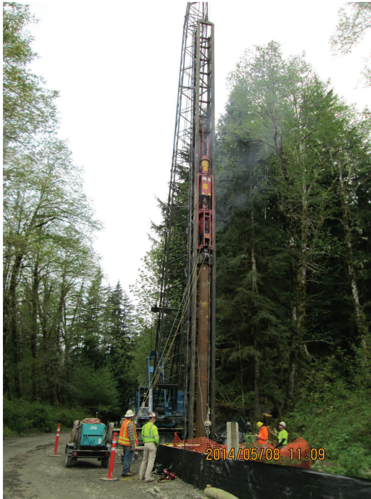
Right: Pile driving at the 588+50 Bridge
