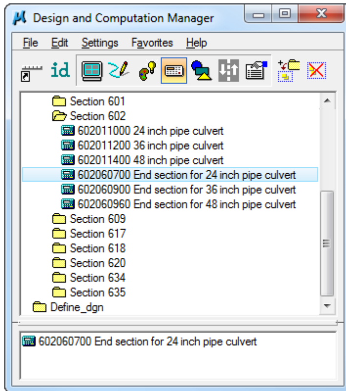
Figure 10.1-1: Item Selection
