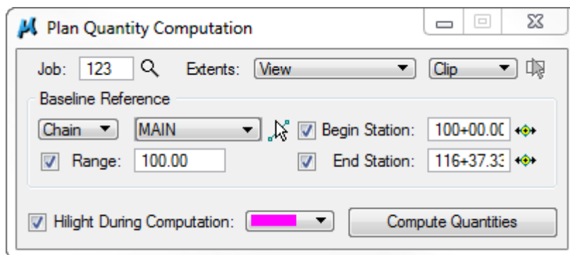
Figure 10.1-2: Compute Dialog
