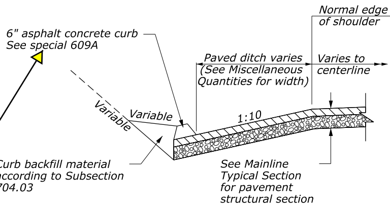
TYPICAL PAVED DITCH SECTION
