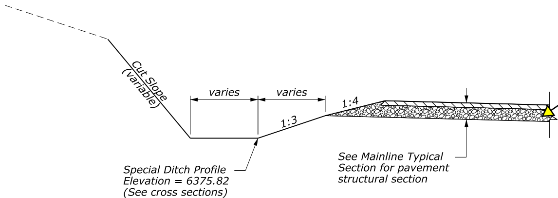
SPECIAL DITCH SECTION
