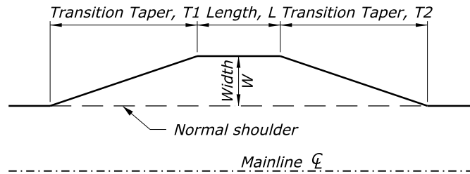
TYPICAL WIDENING AND PULLOUT PLAN
