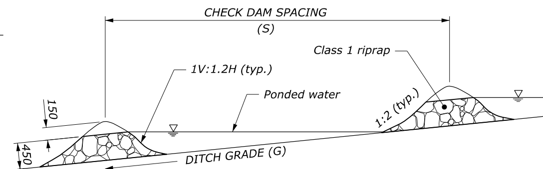
PROFILE VIEW
