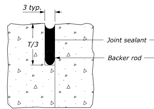
CONSTRUCTION JOINT
