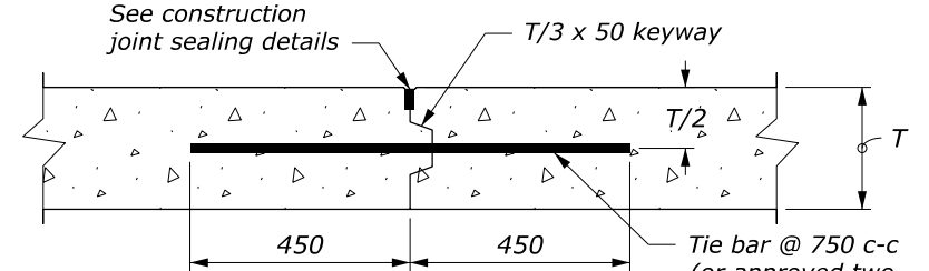
CONSTRUCTION JOINT KEYWAY - LONGITUDINAL
