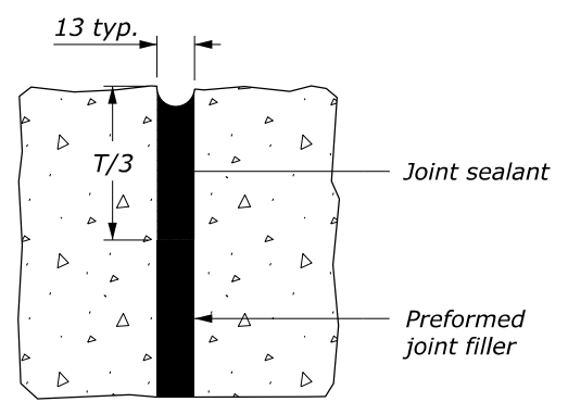
ISOLATION JOINT
