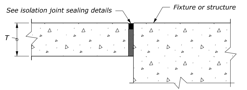
ISOLATION JOINT UNDOWELED - LONGITUDINAL
