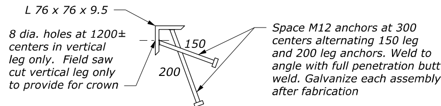
GUARD ANGLE DETAIL (4 required per cattle guard)
