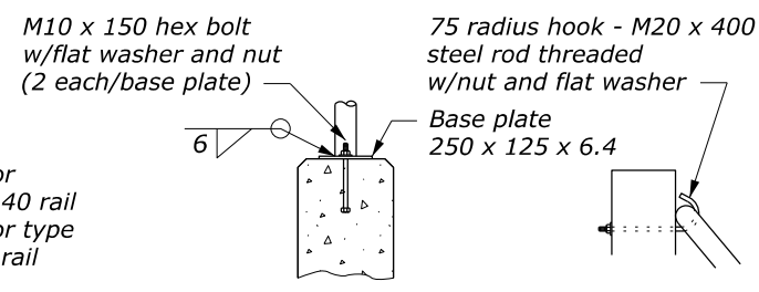
DETAIL E
