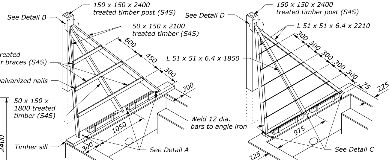
WOOD WING GUARD
