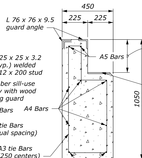
WOOD WING GUARD
