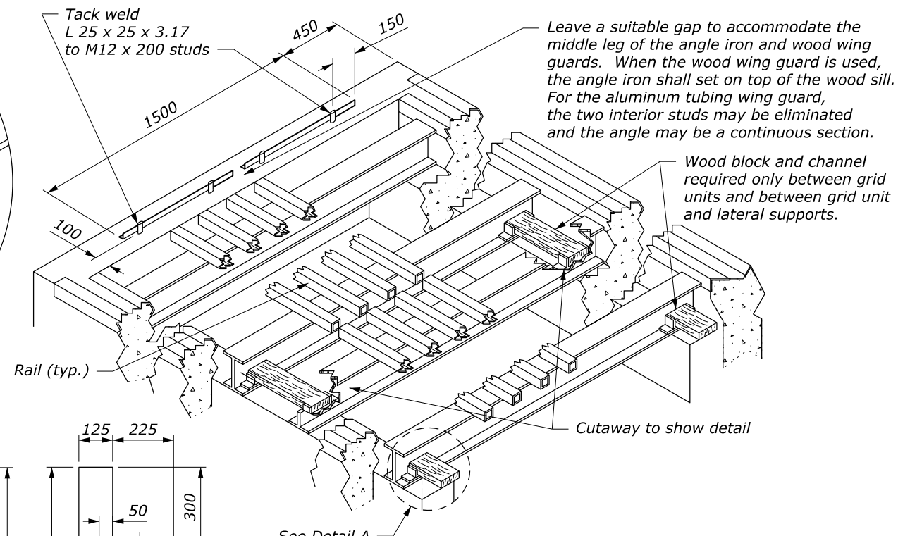
ISOMETRIC VIEW
