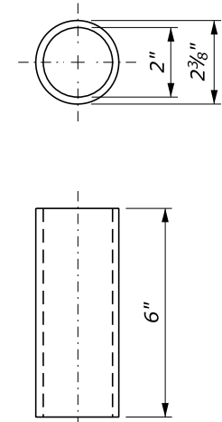
POST SLEEVE
