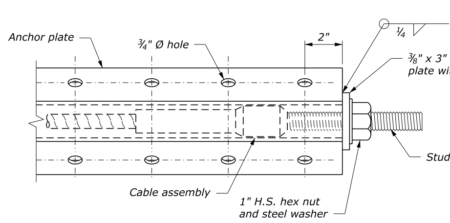
CABLE ANCHOR PLATE DETAILS
