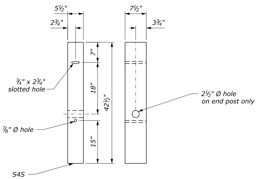
TERMINAL POST
