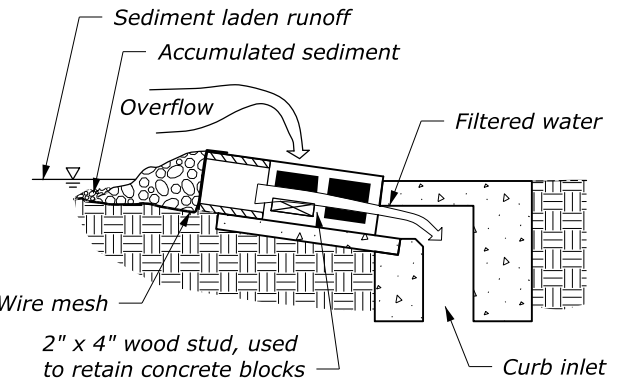
SECTION B-B CURB INLET PROTECTION, BLOCK AND GRAVEL (TYPE D)
