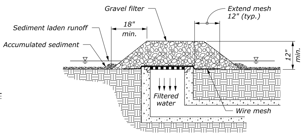
GRAVEL AND WIRE MESH DROP INLET PROTECTION (TYPE B)
