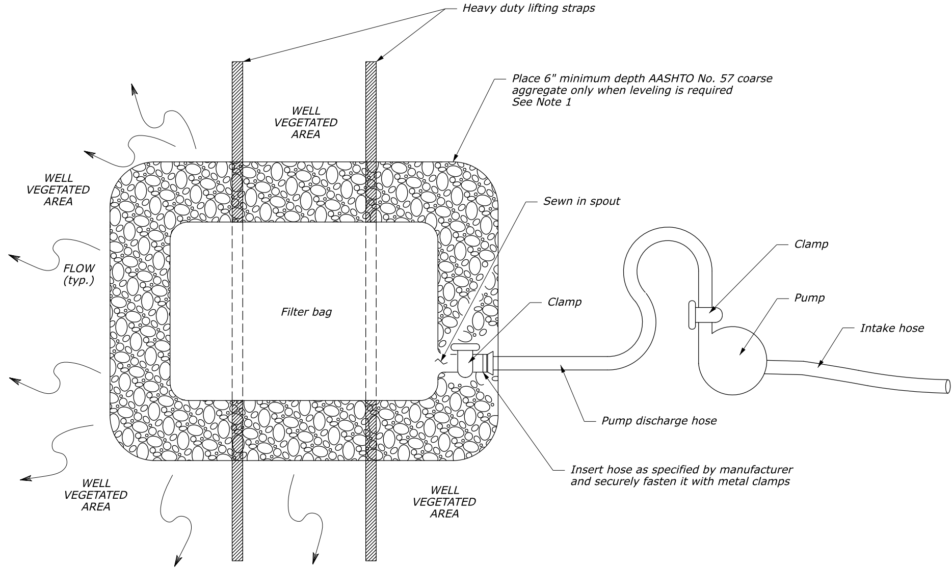
TOP VIEW
