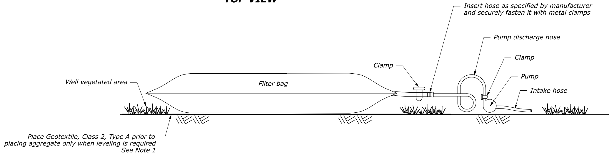
SIDE VIEW
