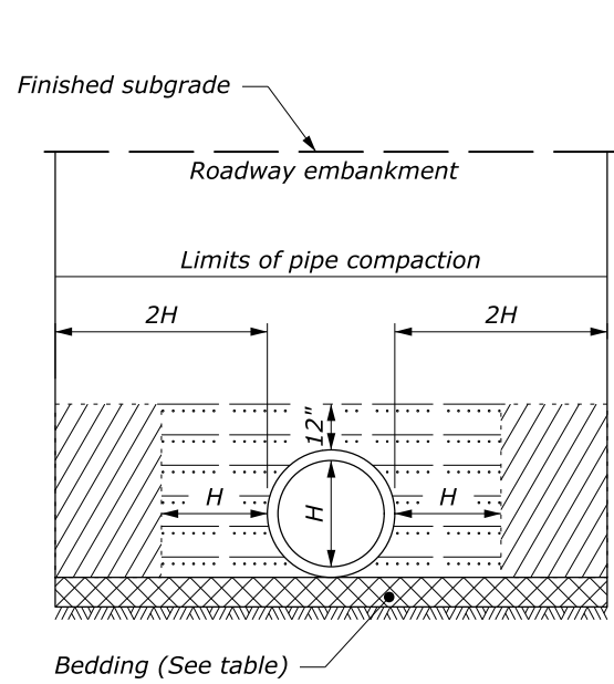
EMBAKMENT INSTALLATION
