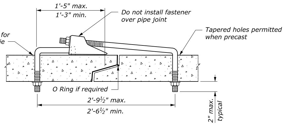
SUPPLEMENTAL CONCRETE PIPE TIE
