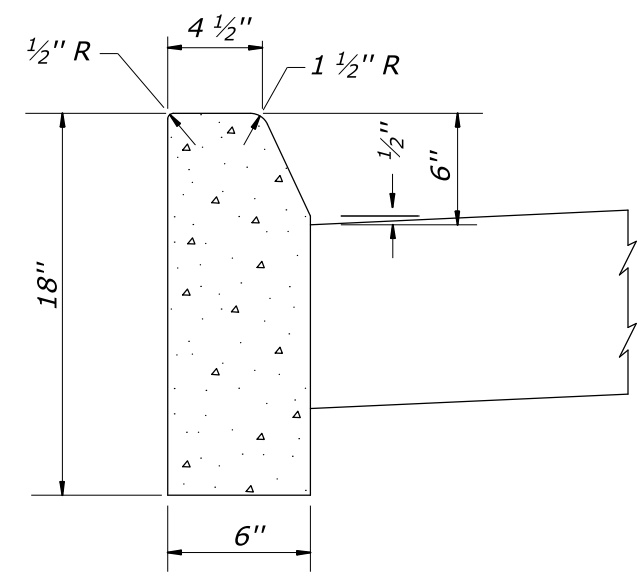
18-INCH DEPTH (NON-MOUNTABLE)
