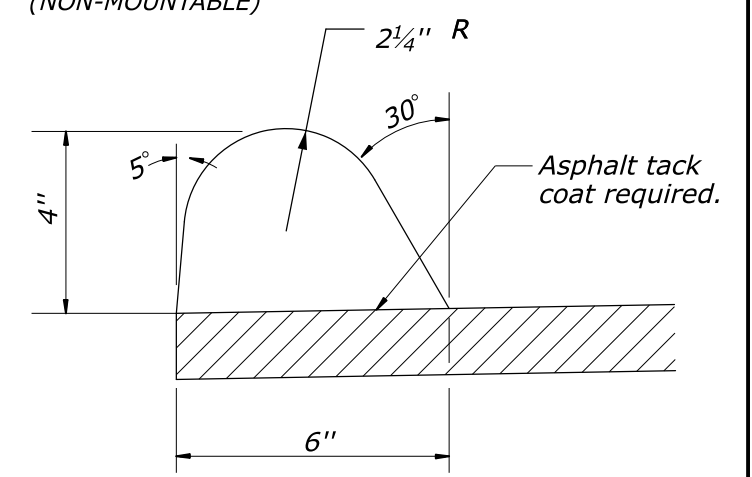
ASPHALT CONCRETE CURB 4-INCH DEPTH (NON-MOUNTABLE)
