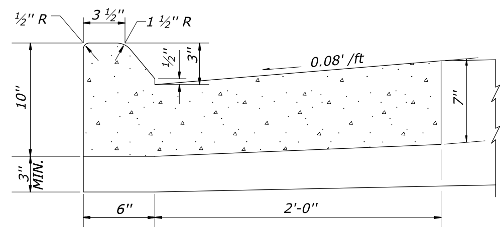
10-INCH DEPTH (MOUNTABLE)
