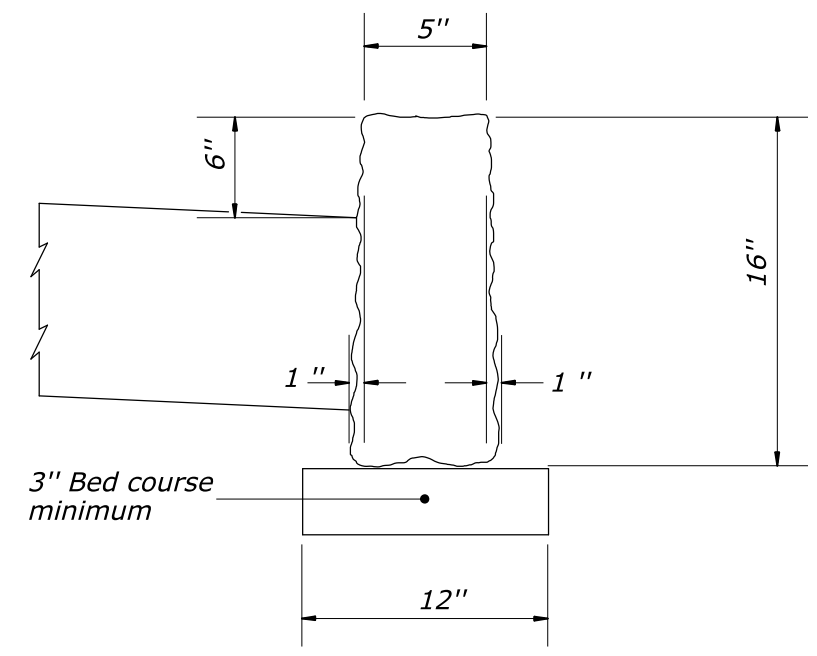
STONE CURB 16-INCH DEPTH (NON-MOUNTABLE)
