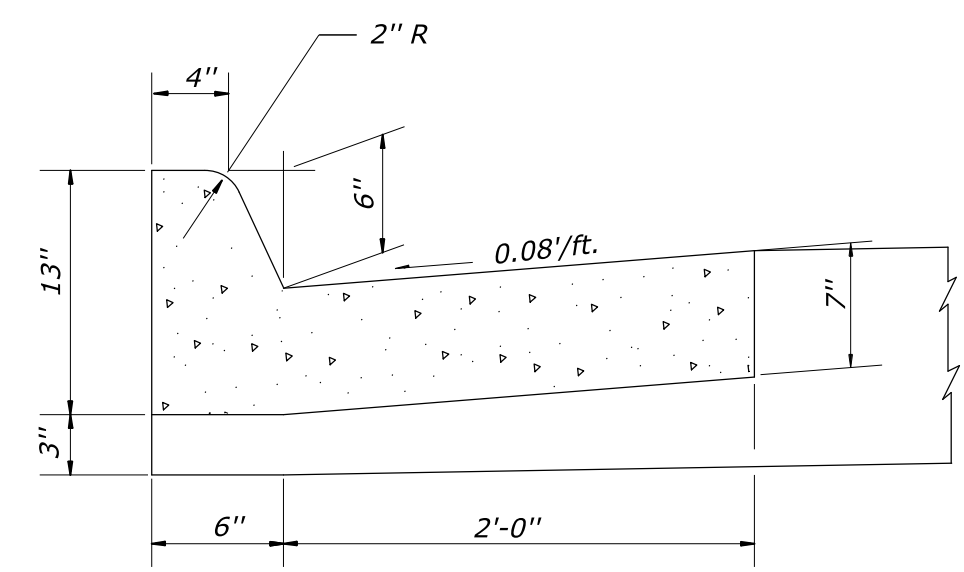
13-INCH DEPTH (NON-MOUNTABLE)
