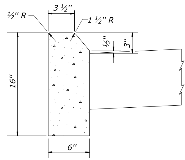
16-INCH DEPTH (MOUNTABLE)
