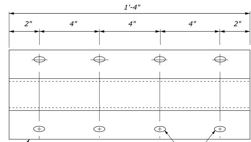
Bent Plate 3/16" thickness
