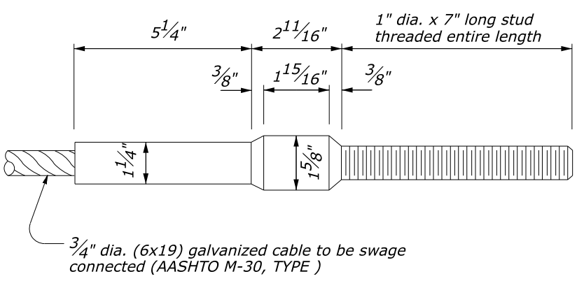
Standard swaged fitting
