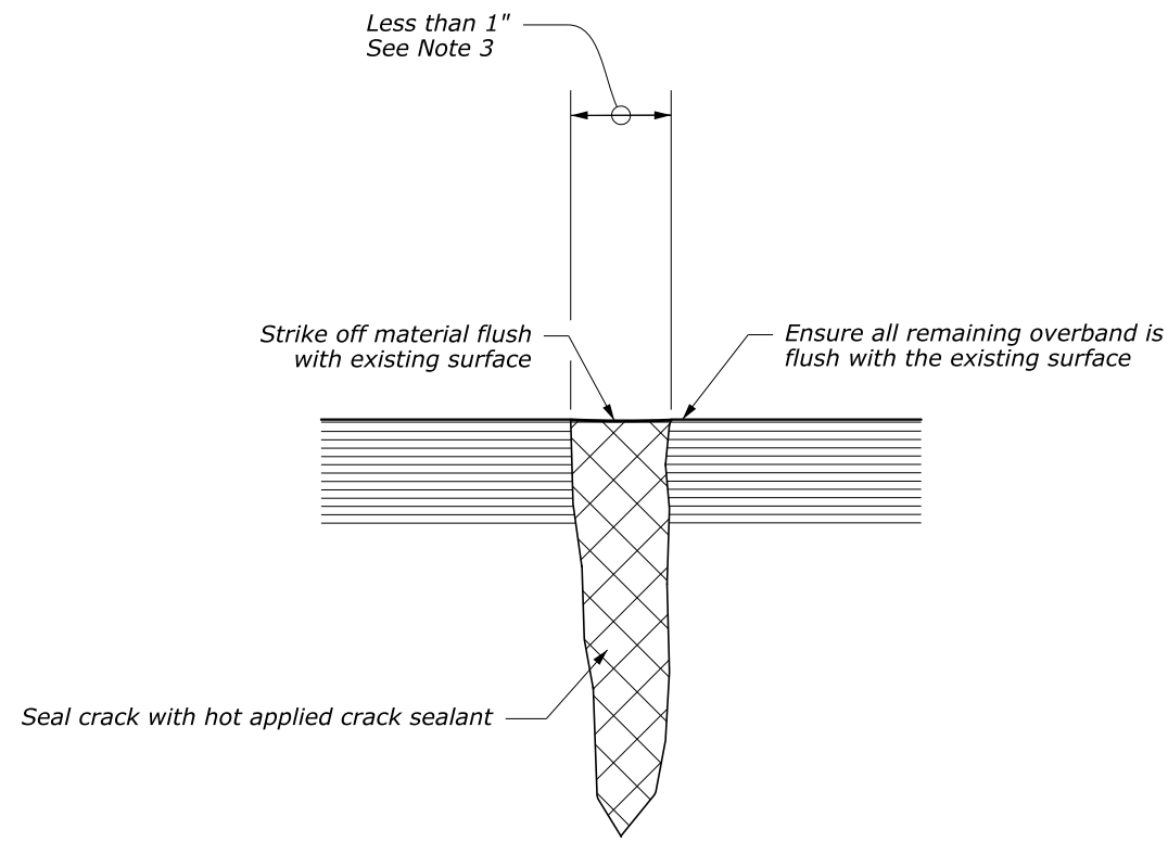
CRACK SEALING
