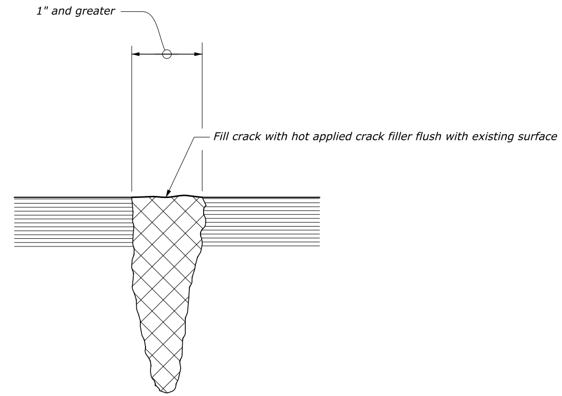
CRACK FILLING
