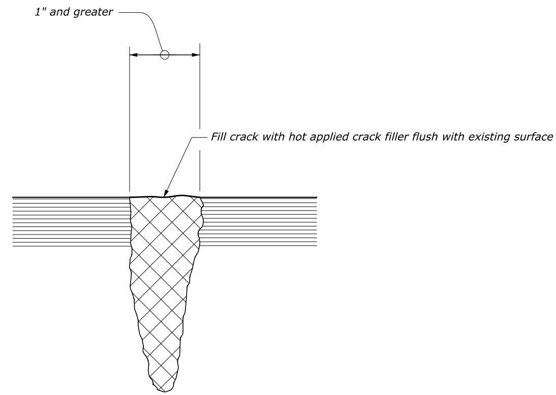
CRACK FILLING
