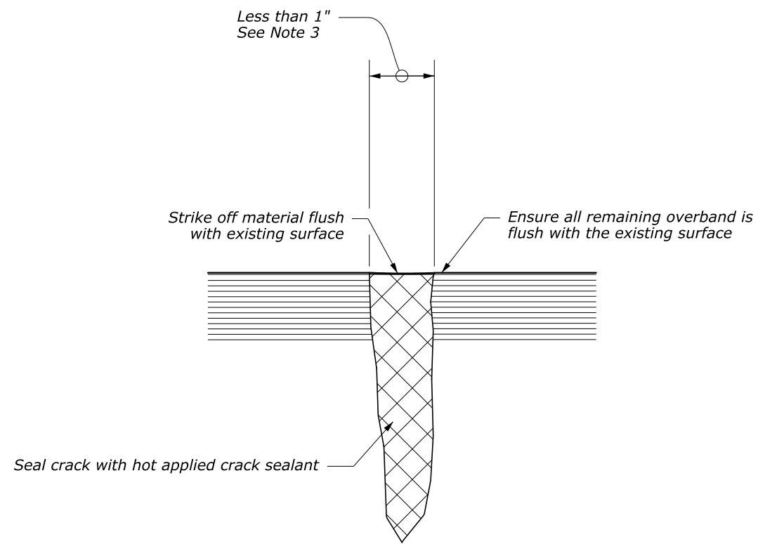
CRACK SEALING
