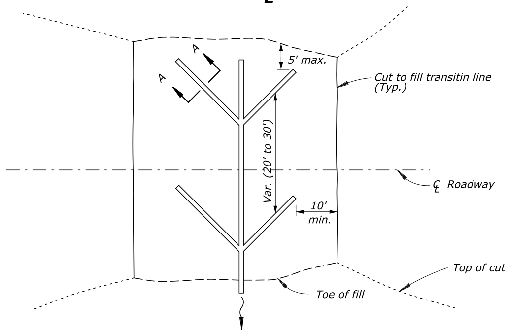
HERRINGBONE DRAINAGE PATTERN (PERPENDICULAR TO \zeta )
