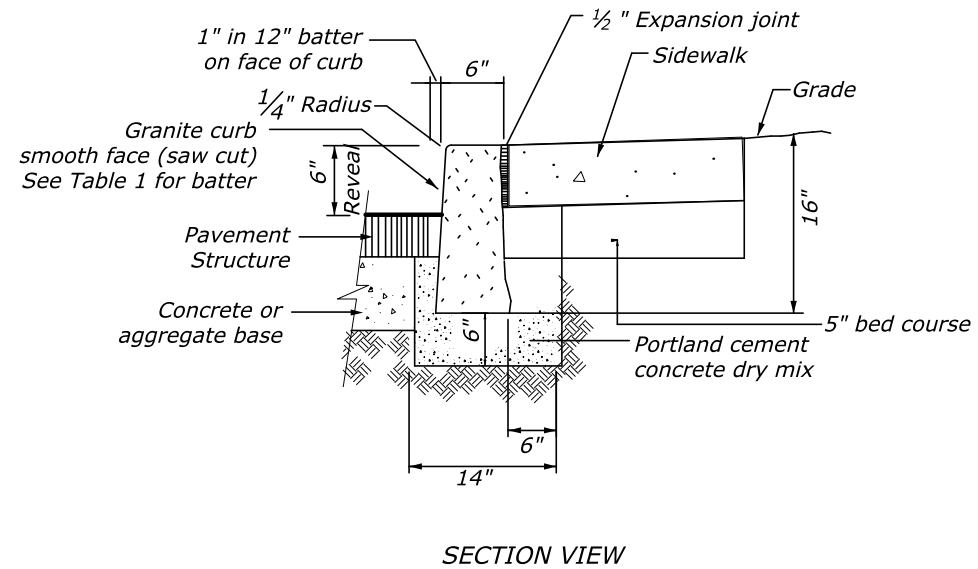
STONE CURB TYPE 1, 16" DEPTH (GRANITE TYPE A OR B) (WITH SIDEWALK)
