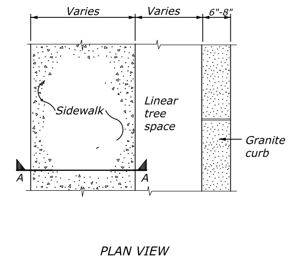
STONE CURB TYPE 1, 16" DEPTH (GRANITE TYPE A OR B) (WITH SIDEWALK AND LINEAR TREE SPACE)
