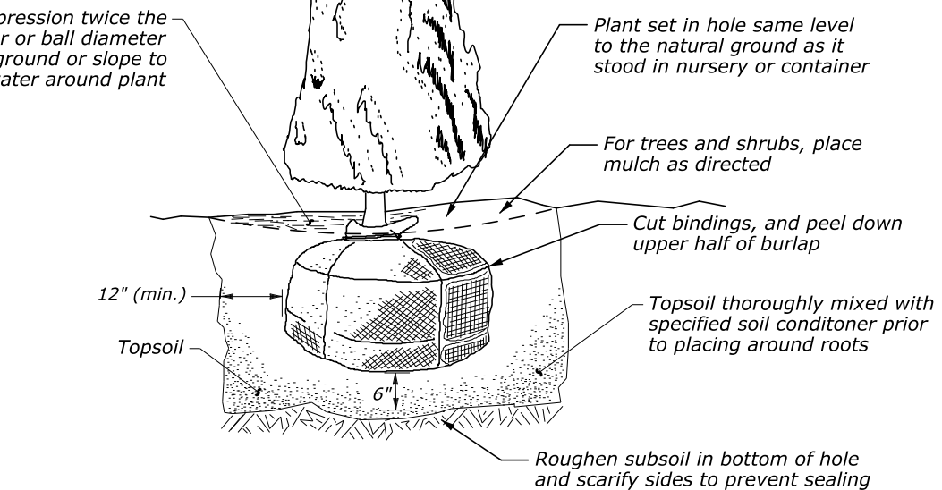
METHOD OF PLANTING CONTAINER OR BALLED AND BURLAPPED TREES AND SHRUBS
