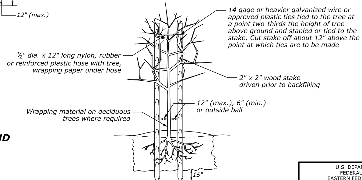
METHOD OF STAKING DECIDUOUS TREES UNDER 12'
